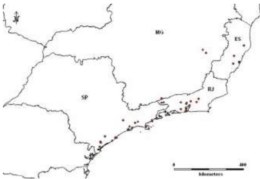
Fig. 58. Distribution of Cryptocarya saligna Mez.
